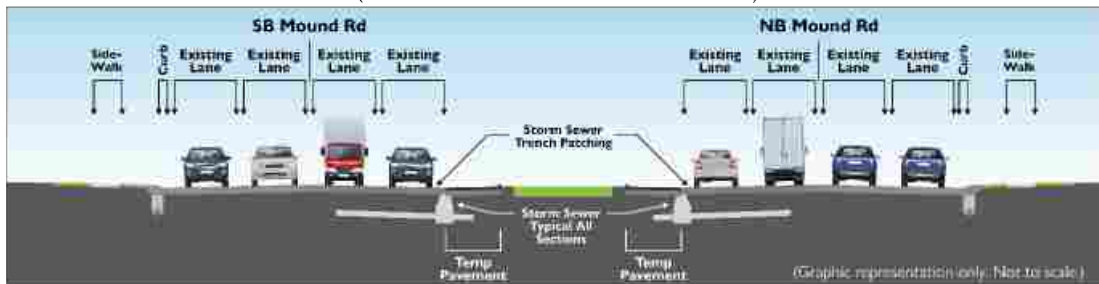
WINTER CONFIGURATION (15 MILE ROAD TO 17 MILE ROAD)
