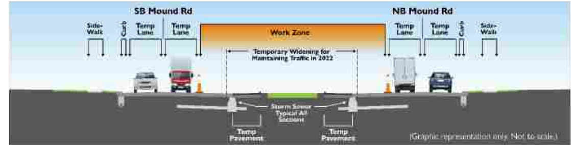
TYPICAL WORK ZONE FOR 2021 CONSTRUCTION (17 MILE ROAD TO M-59)
